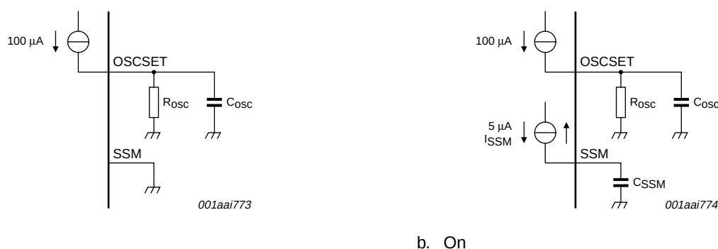
Fig 6. Spread spectrum mode
